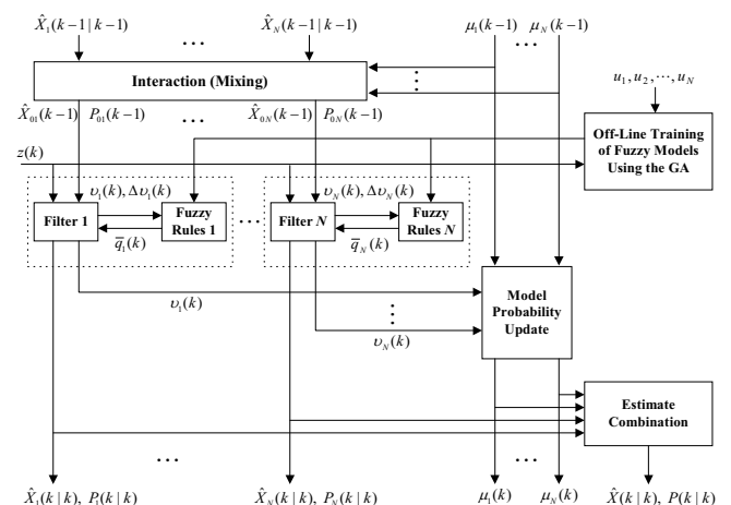
Fig. 2. GA-based IMM method using fuzzy logic.
