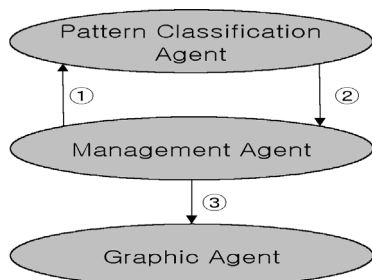
Fig. 4. Management Agent.
